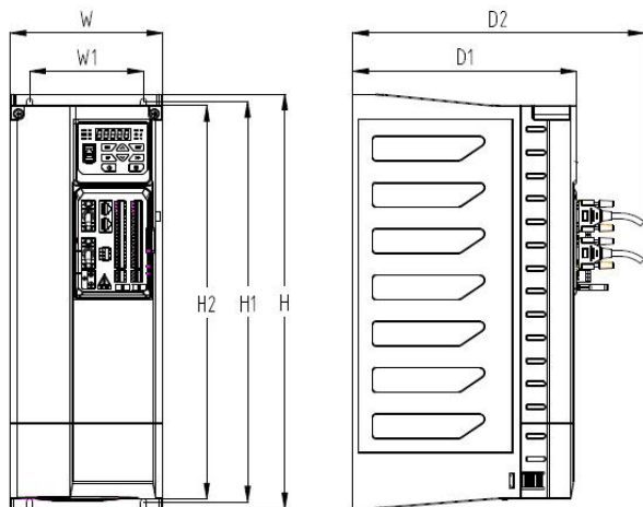
b) GK900-4T18.5LB~GK900-4T45L(B)
