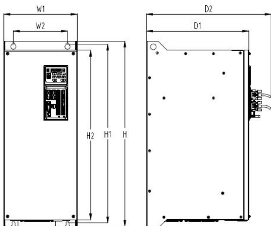
c) GK900-4T55L(B) ~GK900-4T250L
