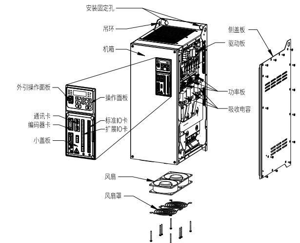
c) GK900-4T55L(B) ~ GK900-4T250L
